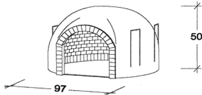
Artigiano80 footprint
