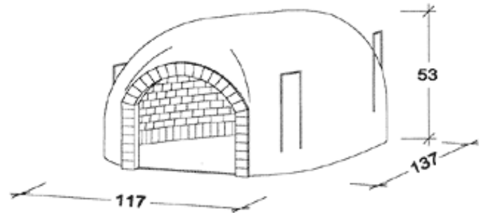
Artigiano120 footprint
